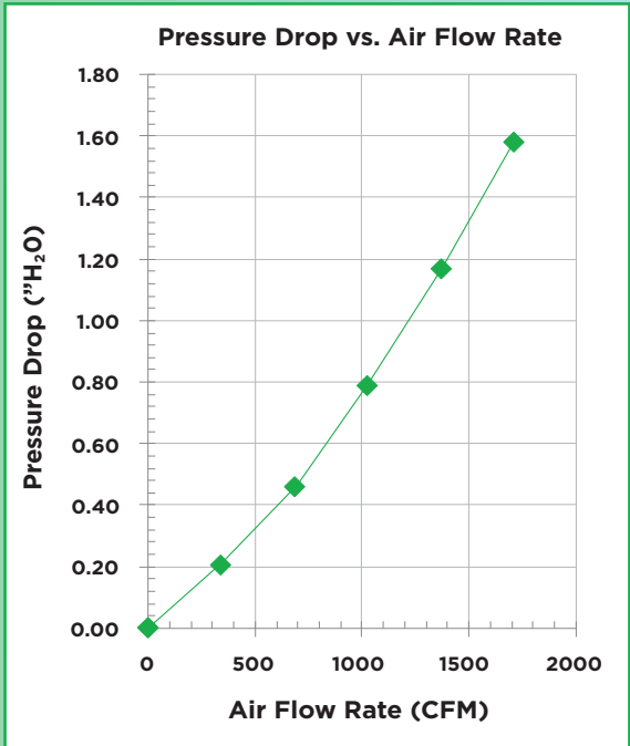
(based on 20x20x4 M13 mini pleat with header)
