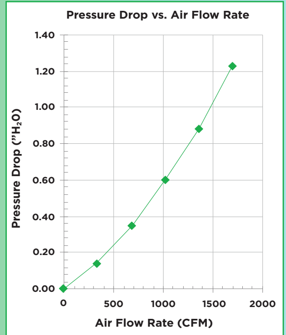
(based on 20x20x4 M15 mini pleat with header)
