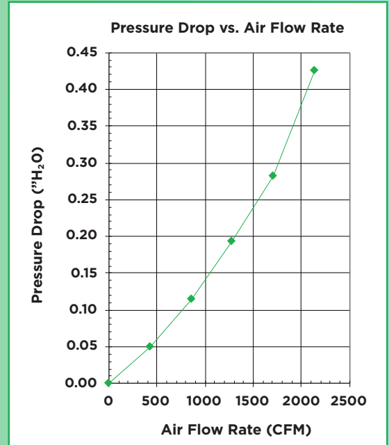
(based on 20x25x5 M13 Whole House Filter)
