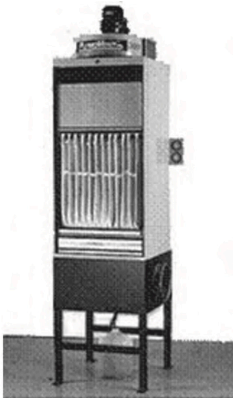
Figure 5: Progressive filtration unit with spark arrester, MERV 14 filter and HEPA final filter configuration. Courtesy Plymovent North America
