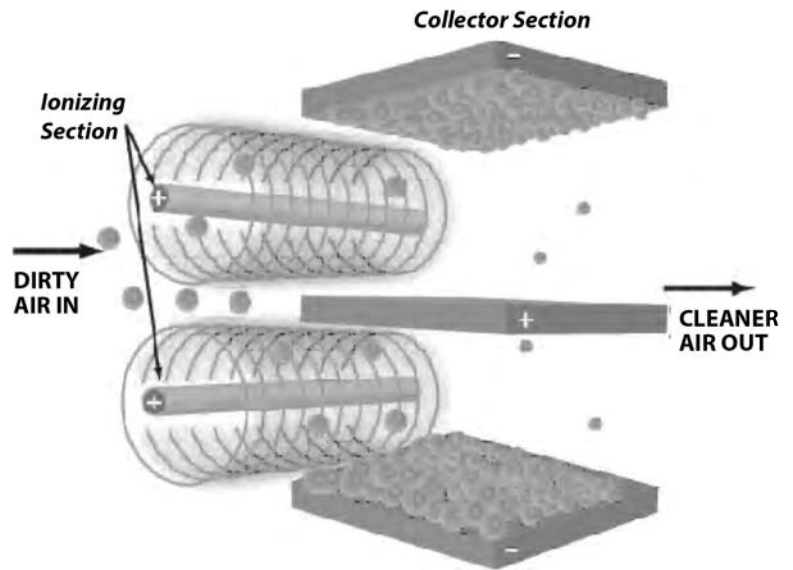
Figure 6: Two-stage electrostatic precipitator (also called an electronic air cleaner). Courtesy Honeywell
