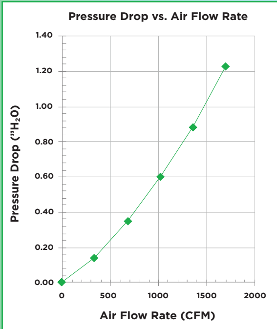
(based on 20x20x4 M14 mini pleat with header)
